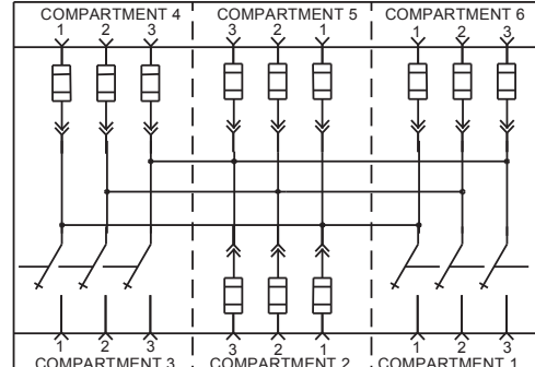
Drawing Number 37-3146-024 – Two opposite incoming switched ways and four fused load ways
