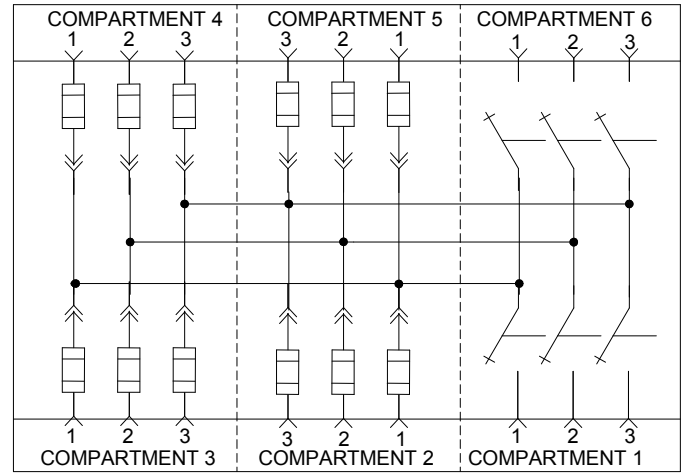
37-3256-003 (PSE-56242) -- Two adjacent switched ways and four fused ways.
